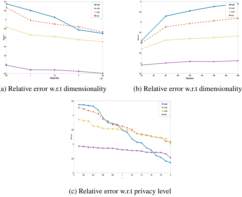
Figure 3: LDP-PCA in low dimensional case on synthetic datasets. The left one is for different target dimensions k over sample size n with fixed \epsilon = 0.5 and p = 40 . The middle one is for different dimensions with fixed n = 10^5 and \epsilon = 0.5 . The right one is for different level of privacy with fixed n = 10^5 and p = 40 .
