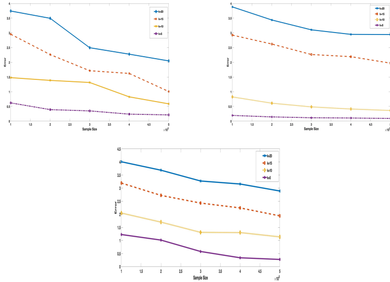
Figure 1: LDP-PCA in low dimensional case on real world datasets with different sample size. The left one is for Coverttype. The middle one is for Buzz. The right one is for Year dataset.
