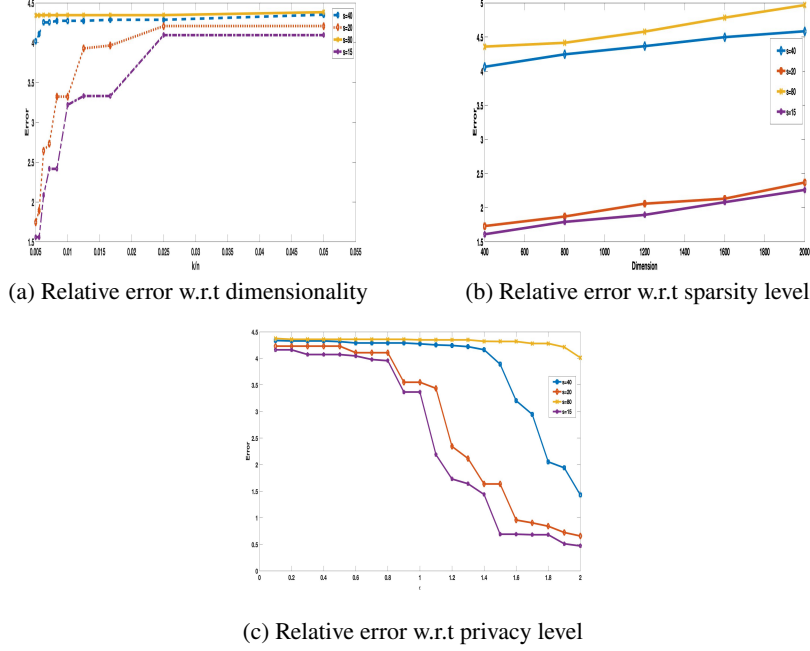
Figure 4: LDP-PCA in high dimensional case on synthetic datasets. The left one is for different target dimensions k over sample size n with fixed \epsilon = 1 and p = 400 . The middle one is for different dimensions with fixed n = 2000 and \epsilon = 1 . The right one is for different level of privacy with fixed n = 2000 and p = 400 .
